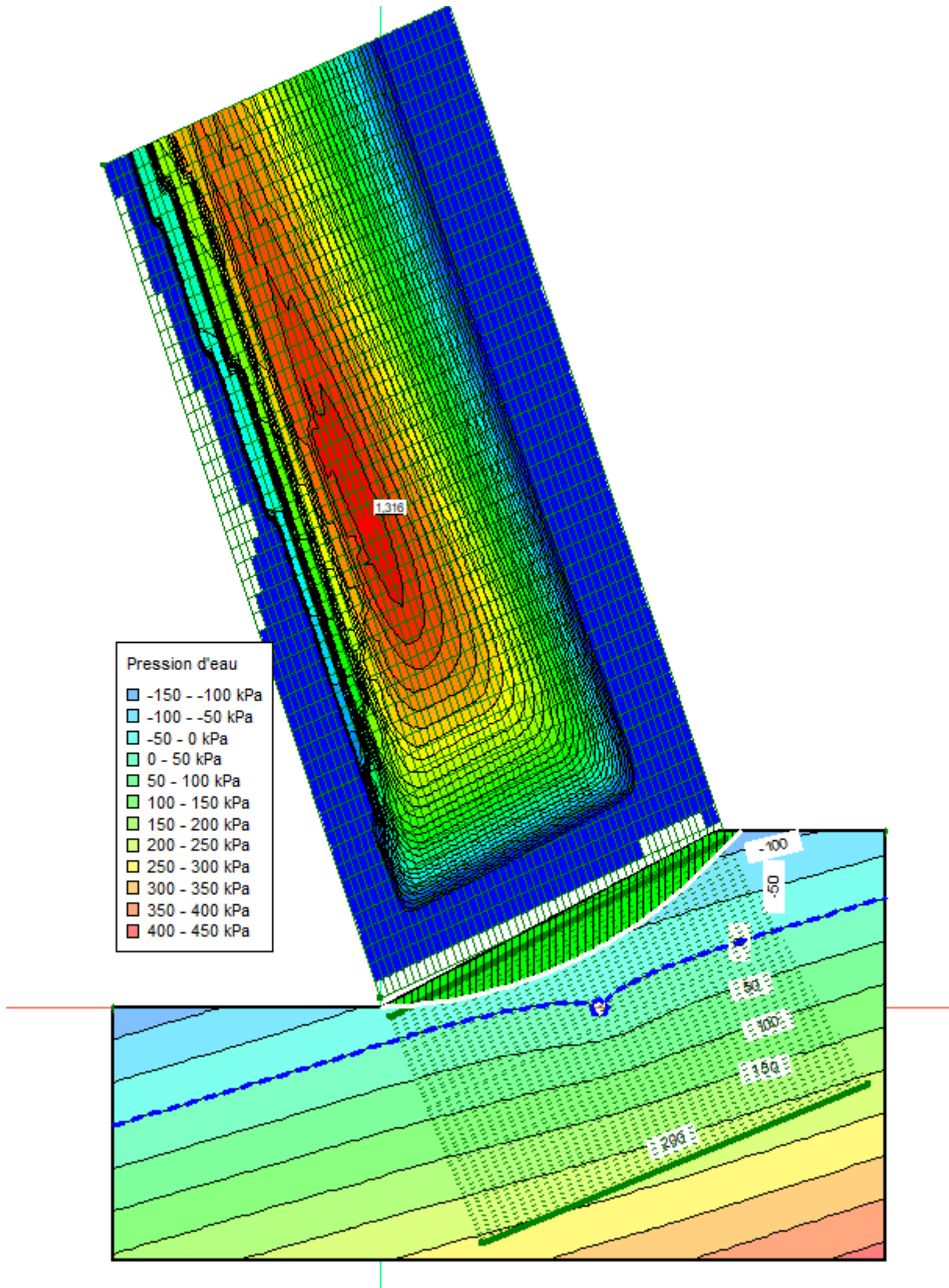
Figure 7: Pore water pressure map contour and safety factor identification (model with gallery).
