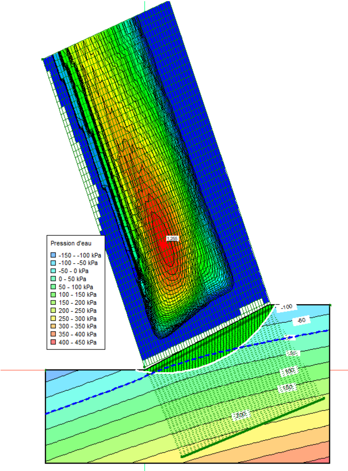
Figure 5: Pore water pressure map contour and safety factor identification (model without gallery).
