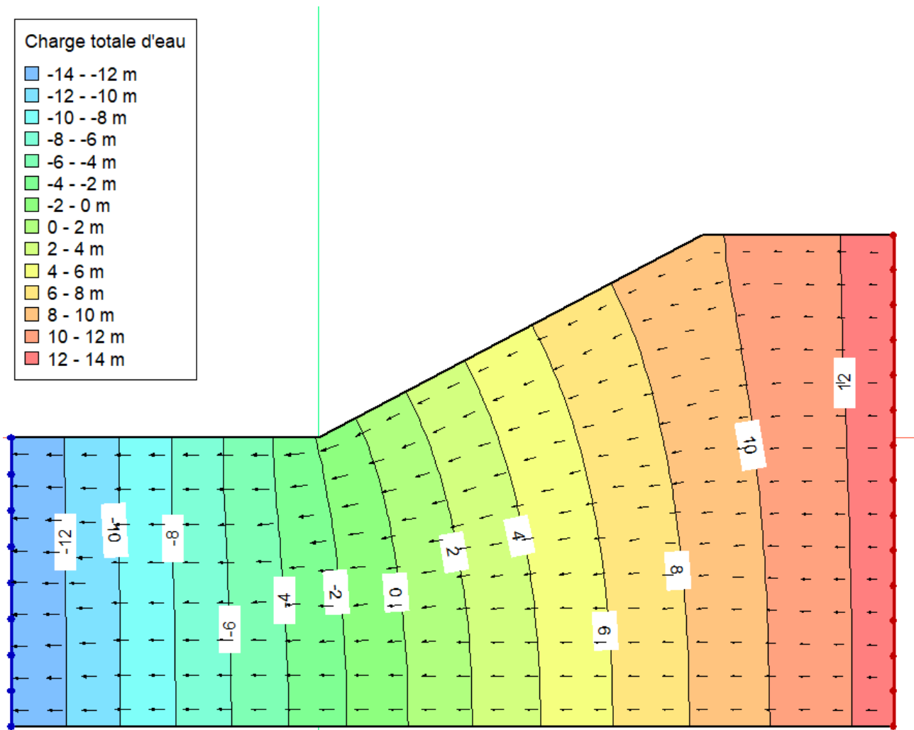
Figure 4: Water total head map contour (model without gallery).
