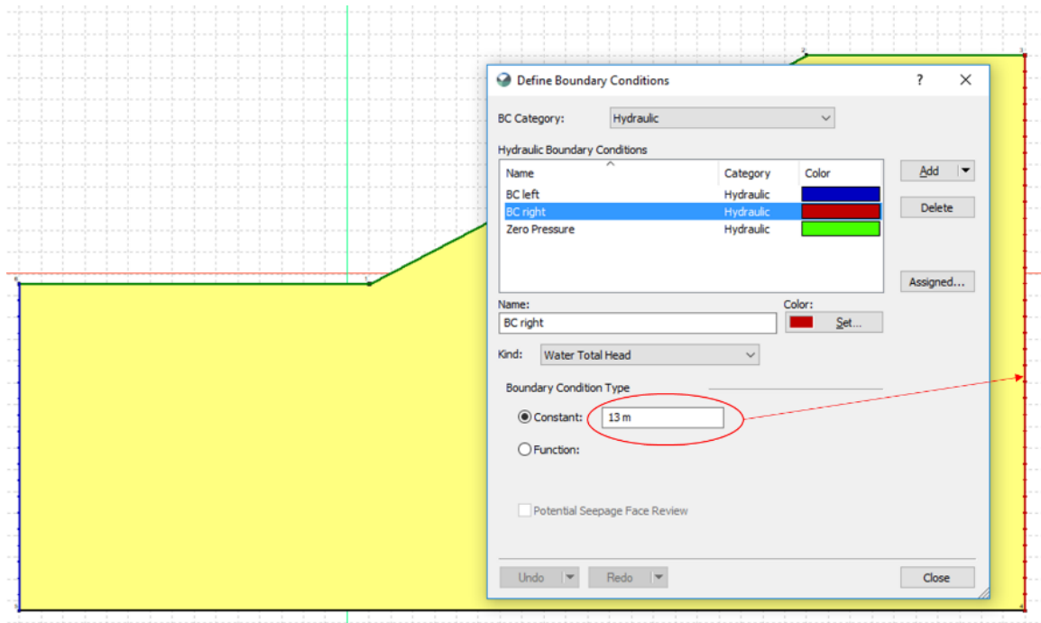
Figure 2: The hydraulic boundary conditions to be applied.
